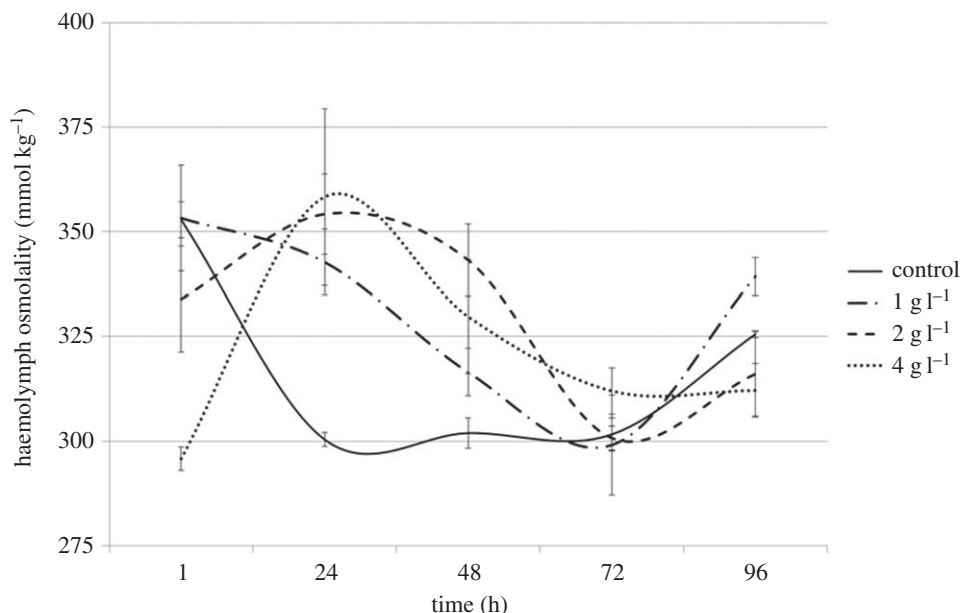
Figure 2. Temporal variability in mean haemolymph osmolality ( \pm s.e.m., n = 3 ) of the mayfly nymph Austrophlebioides pusillus at constant salinities of 1, 2 and 4 \text{g l}^{-1} added SMS.
