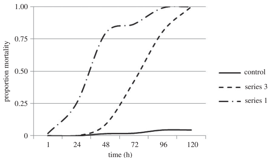
Figure 4. Comparison of mortality for Austrophlebioides pusillus under direct transfer (series 1) and ramp increase (series 3) salinity exposures. Series 1 = A. pusillus in aquarium salinity of 10 g l -1 SMS. Series 3 = A. pusillus as aquarium salinity is gradually increased to 10 g l -1 SMS over a 72 h period and maintained at this concentration for a further 48 h. Data are means \pm s.e.m., n = 3 .
